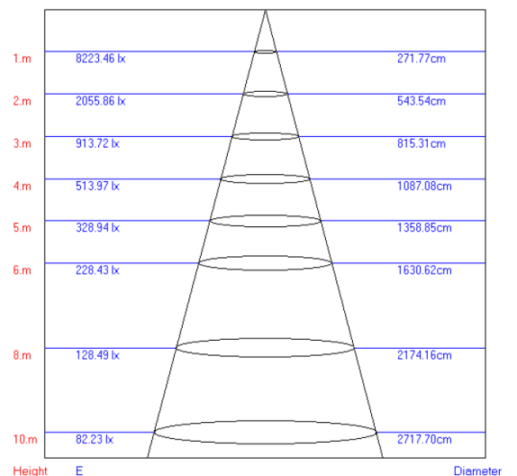
Lux-Distance Curve
